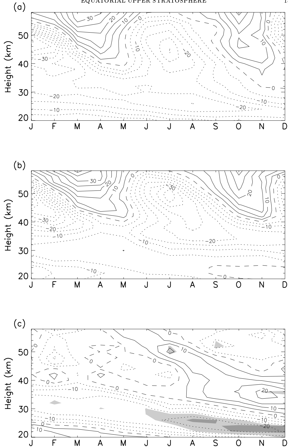
Figure 11. Time-series of monthly-averaged u_{eq} ( ms^{-1} ) measured by rocketsonde. (a) Composite of 5 warmest NH winters, as determined using 30 hPa NP temperatures, (b) As for panel (a) but for the 5 coldest winters. (c) The difference between the two composites i.e. panel (a) minus panel (b). Contour interval is 5 ms^{-1} . Negative (easterly) values are denoted by dotted contours. Light and dark shading denote regions where values are significant at the 95% and 99% confidence levels respectively. The significances of the values were tested by performing a Student's t-test on the difference between the two mean wind distributions.
