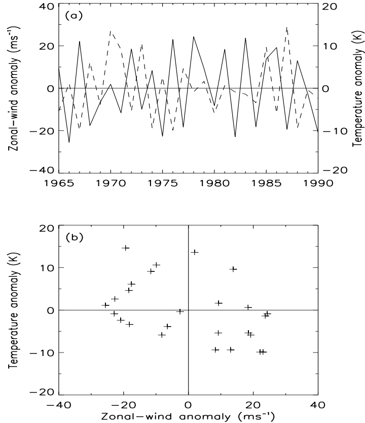
Figure 2. (a) Time-series of JF NP temperature anomalies (K) at 24 km ( \sim 30\text{hPa} ) (dotted line) and u_{\text{eq}} anomalies ( \text{ms}^{-1} ) at 24 km in the preceding December (solid line). (b) Scatter plot of the data.
