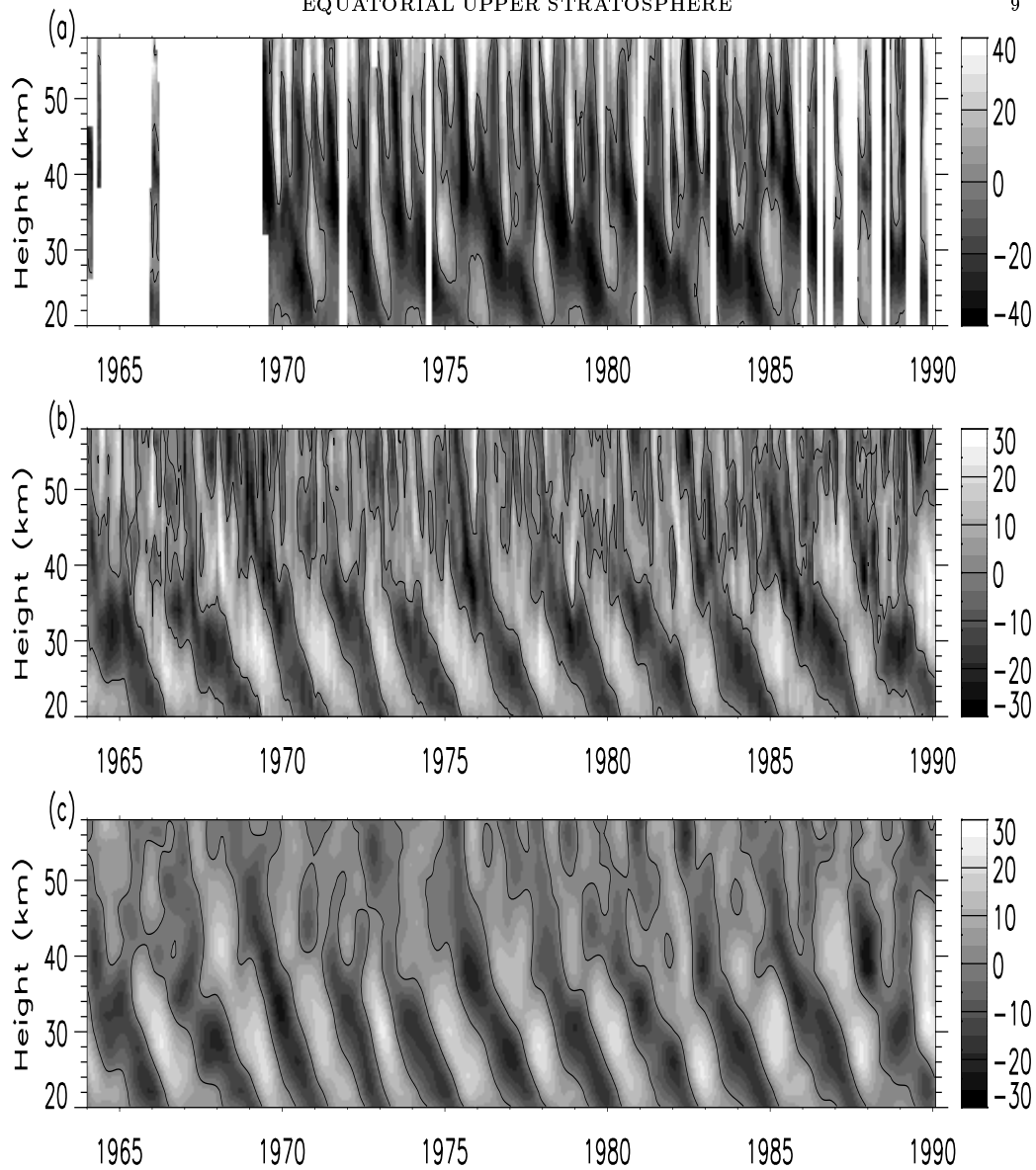
Figure 6. (a) Monthly-averaged zonal wind ( \text{ms}^{-1} ) derived from rocketsonde ascents at Kwajalein ( 8^{\circ}\text{N} ). (b) De-seasonalised monthly-averaged zonal wind dataset derived by combining data from both Kwajalein and Ascension Island as described in the text. (c) As in panel (b) after passing through a 9-60 month bandpass filter. Zero value is denoted by contour line.
