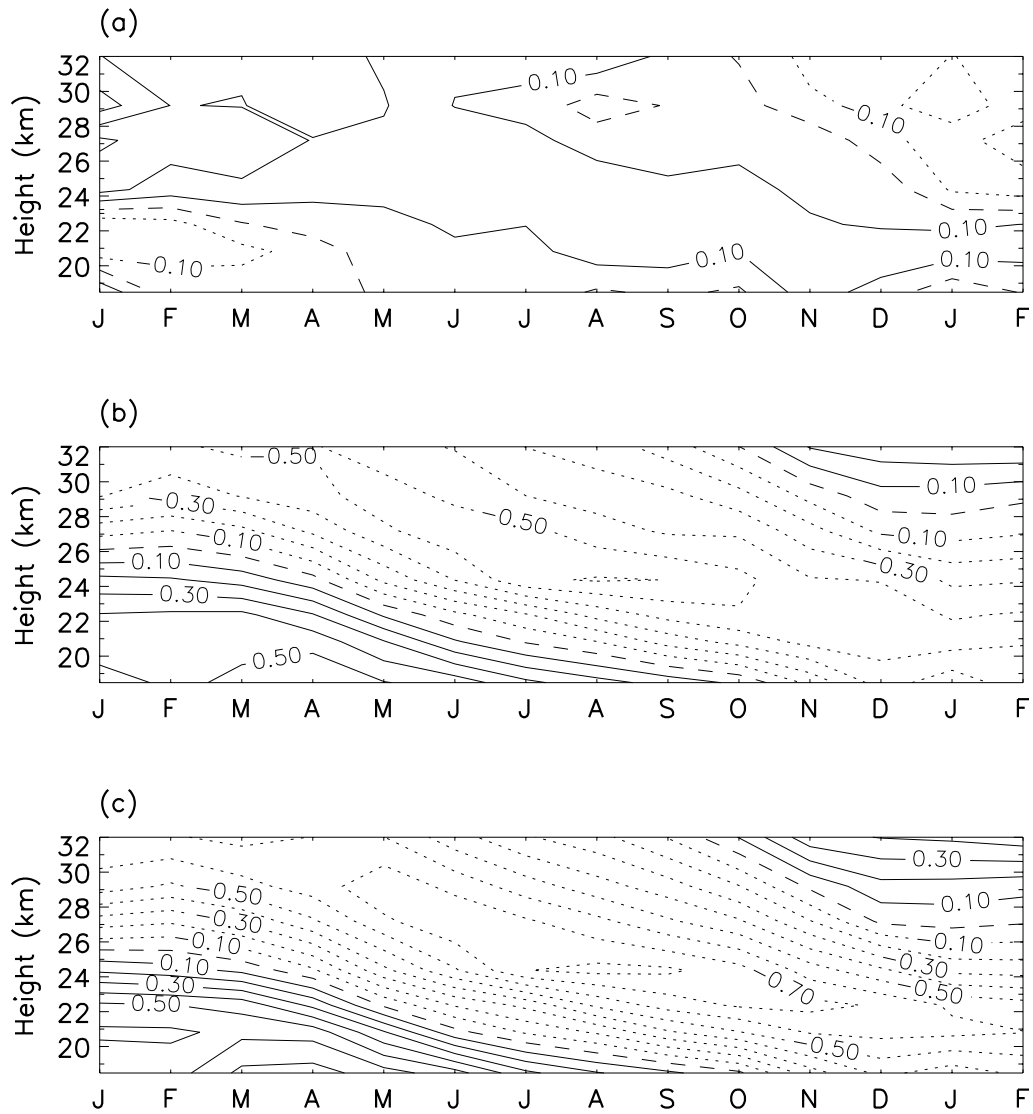
Figure 5. Correlation over the time interval 1955-99 between JF NP temperatures at 24 km and monthly-averaged u_{eq} from radiosonde ascents in each month from January of the previous year to February of the same year. (a) solar maximum years, (b) solar minimum years, (c) solar minimum years but for time interval 1955-96 only. Contour interval is 0.1. Dotted contours denote negative values. Dashed line is zero contour. Note that no confidence levels are estimated as the sampling interval varies in these stratified datasets and hence the autocorrelation of the data cannot be determined (see appendix A)
