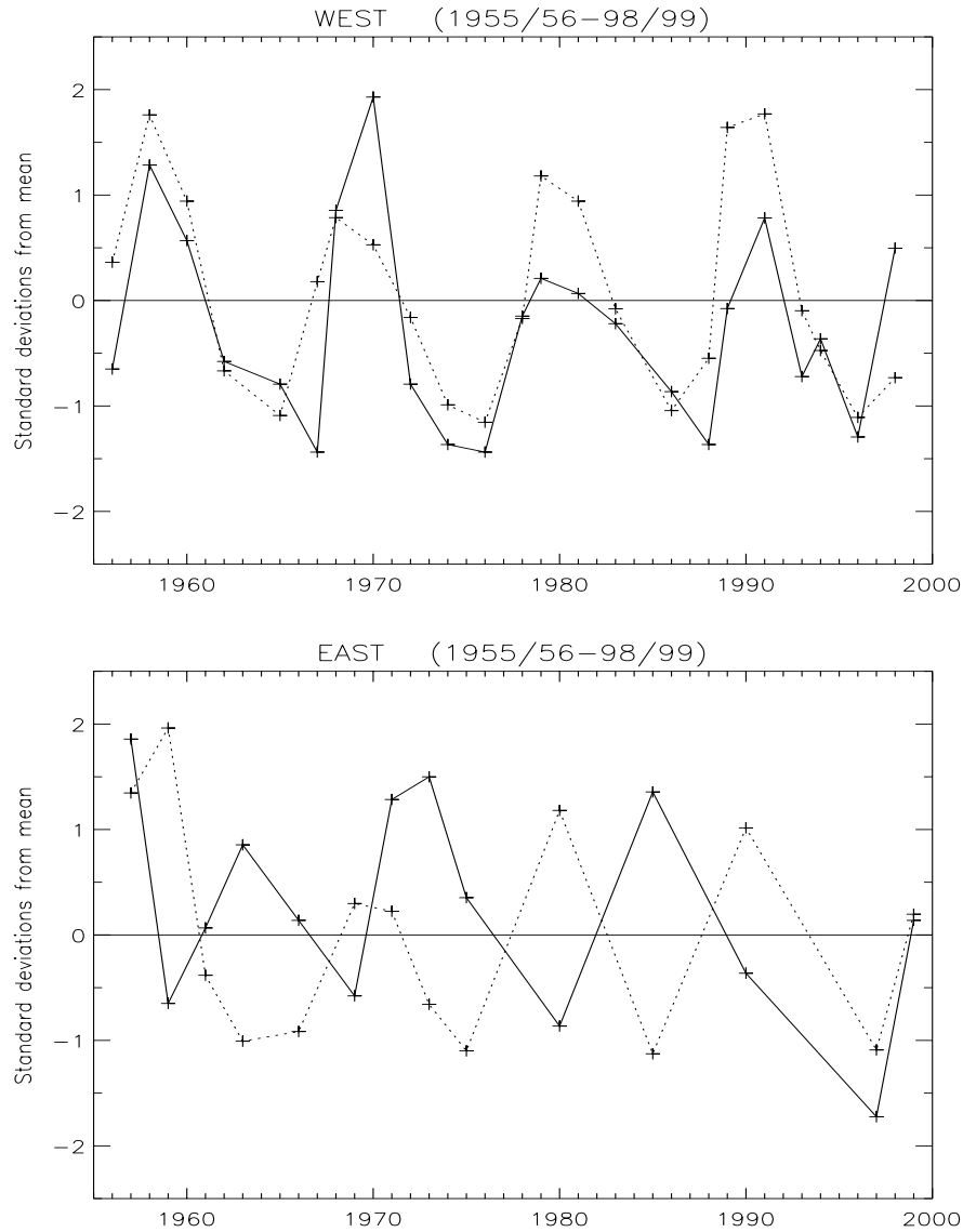
Figure 4. (a) Time series of NP temperature anomaly at 24 km ( \sim 30 hPa) (solid line) and 10.7 cm radio flux (dotted line). (a) west QBO phase years, (b) east phase years. Both signals have been plotted as standard deviations from the mean over the whole time-interval to aid comparison.
