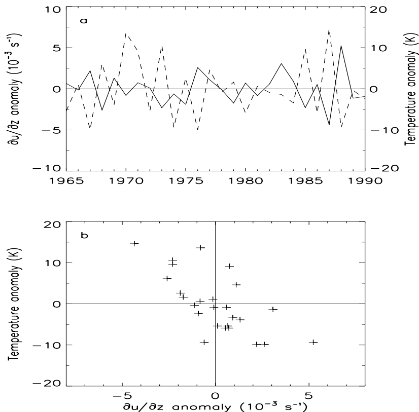
Figure 9. (a) Time-series of JF NP temperature anomalies (K) at 24 km ( \sim 30 hPa) (dotted line) and \partial u_{eq}/\partial z anomalies ( \times 10^{-3} s^{-1} ) at 50 km in the preceding September (solid line). (b) Scatter plot of the data.
