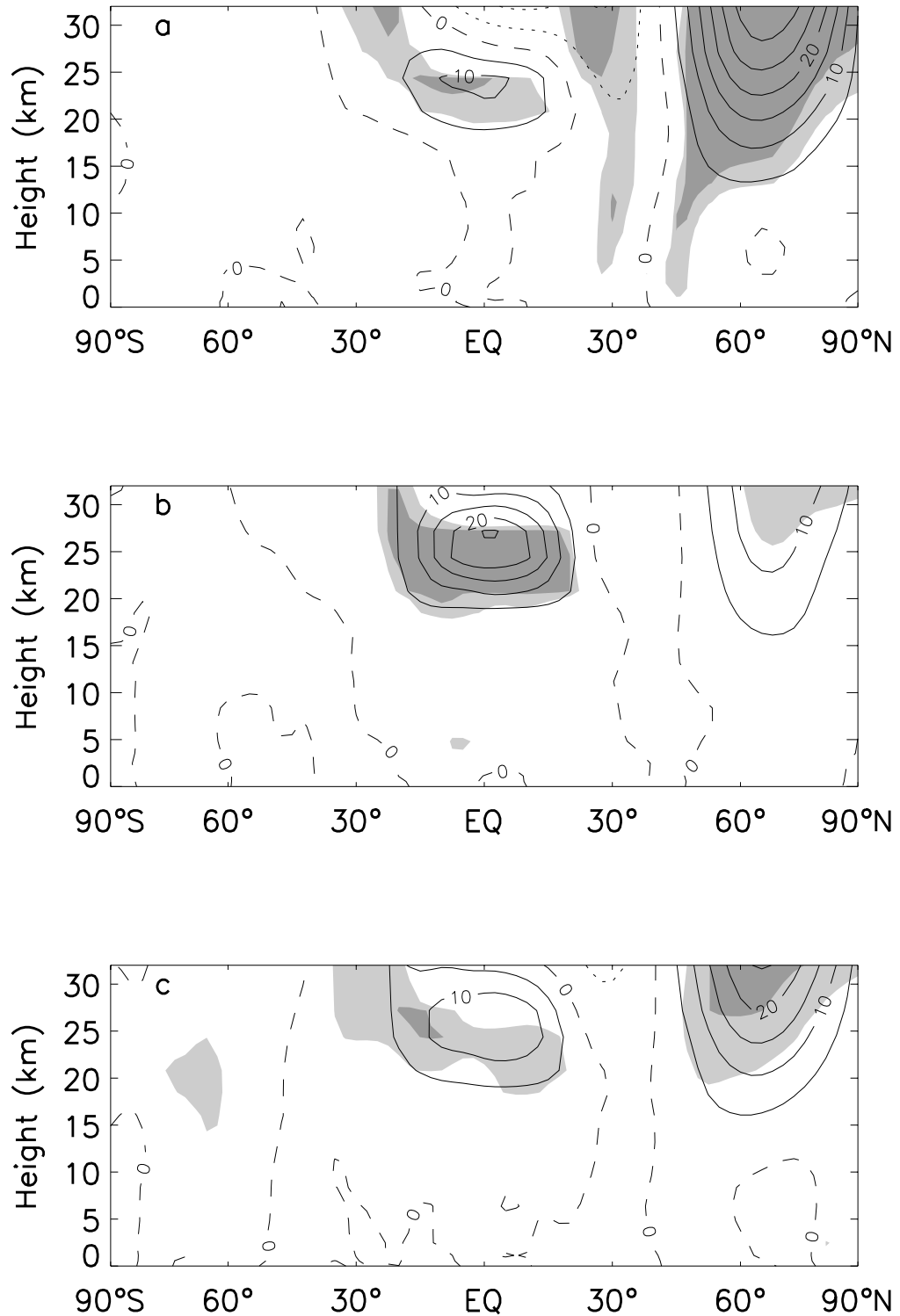
Figure 10. Latitude-height distributions of JF zonally-averaged zonal wind ( \text{ms}^{-1} ) from the NCEP analyses for the period 1964-90. (a) composite difference of the 5 coldest minus 5 warmest NH winters as determined by the 30 hPa JF NP temperatures, (b) composite difference of 5 most westerly minus 5 most easterly QBO phase based on u_{\text{eq}} at 24 km in the previous December, (c) composite difference of 5 strongest minus 5 weakest \partial u_{\text{eq}}/\partial z at 50 km in the previous September. Contour interval is 5 \text{ ms}^{-1} . Negative (easterly) values are denoted by dotted contours. Light and dark shading denote regions where values are significant at the 95% and 99% confidence levels respectively. The significances of the values were tested by performing a Student's t -test on the difference between the two mean wind distributions.
