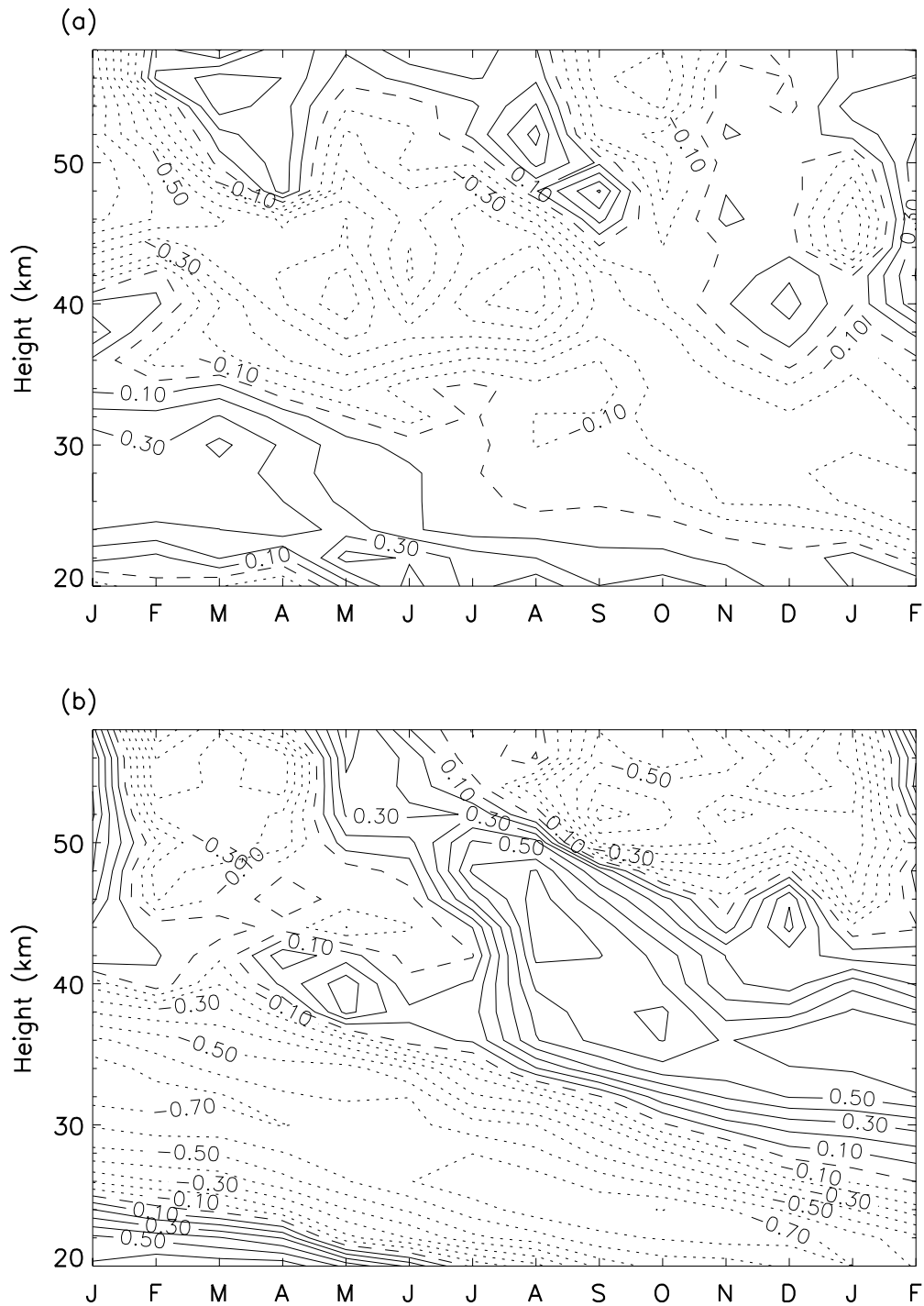
Figure 8. Correlation for the period 1964-90 between JF NP temperatures at 24 km and monthly-averaged u_{eq} from rocketsonde ascents in each month from January of the previous year to February of the same year. (a) solar maximum conditions, (b) solar minimum conditions. Contour interval is 0.1. Dotted contours denote negative values. Dashed line is zero contour. Note that no confidence levels are estimated as the sampling interval varies in these stratified datasets and hence the autocorrelation of the data cannot be determined (see appendix A)
