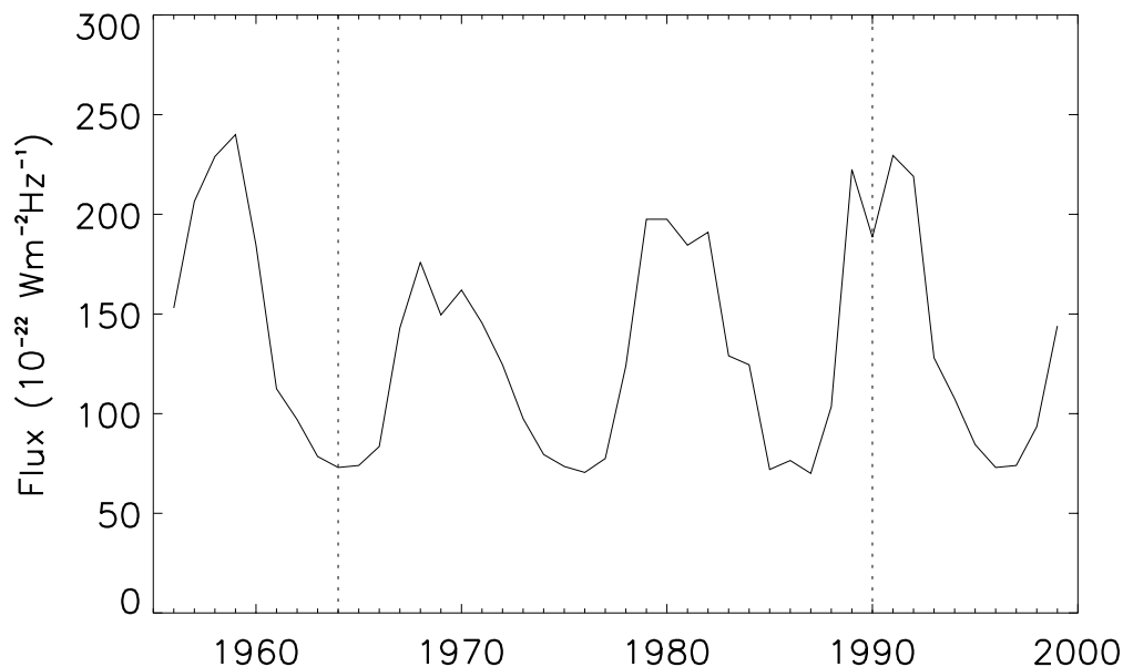
Figure 3. (a) Time-series of annual mean solar 10.7 cm radio flux ( \times 10^{-22} \text{W m}^{-2} \text{Hz}^{-1} ). The dotted lines show the start and end of the period for which the rocketsonde data are available.
