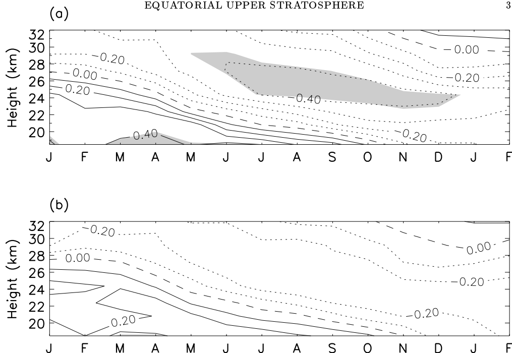
Figure 1. Correlation for the periods (a) 1964-90 and (b) 1955-99 between JF NP temperatures at 24 km and monthly-averaged u_{eq} from radiosonde ascents in each month from January of the previous year to February of the same year. Contour interval is 0.1. Dotted contours denote negative values. Dashed line is zero contour. Shading indicates values are significant at the 95% confidence level (no values were significant at the 99% confidence level). For details of the significance test applied, see appendix A.
