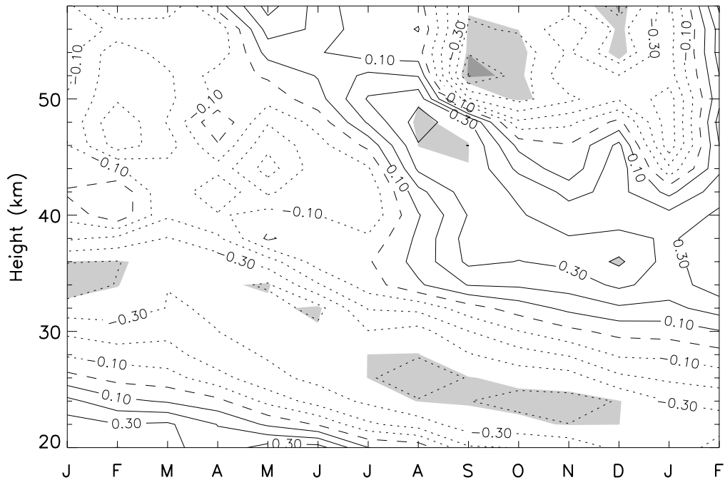
Figure 7. Correlation for the period 1964-90 between JF NP temperatures at 24 km and monthly-averaged u_{eq} from rocketsonde ascents in each month from January of the previous year to February of the same year. Contour interval is 0.1. Dotted contours denote negative values. Dashed line is zero contour. Shading indicates values are significant at the 95% confidence level (no values were significant at the 99% confidence level). For details of the significance test applied, see appendix A.
